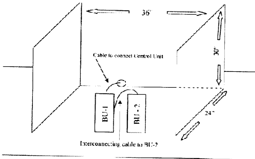
CASCADING OF TWO BALLOT UNITS
